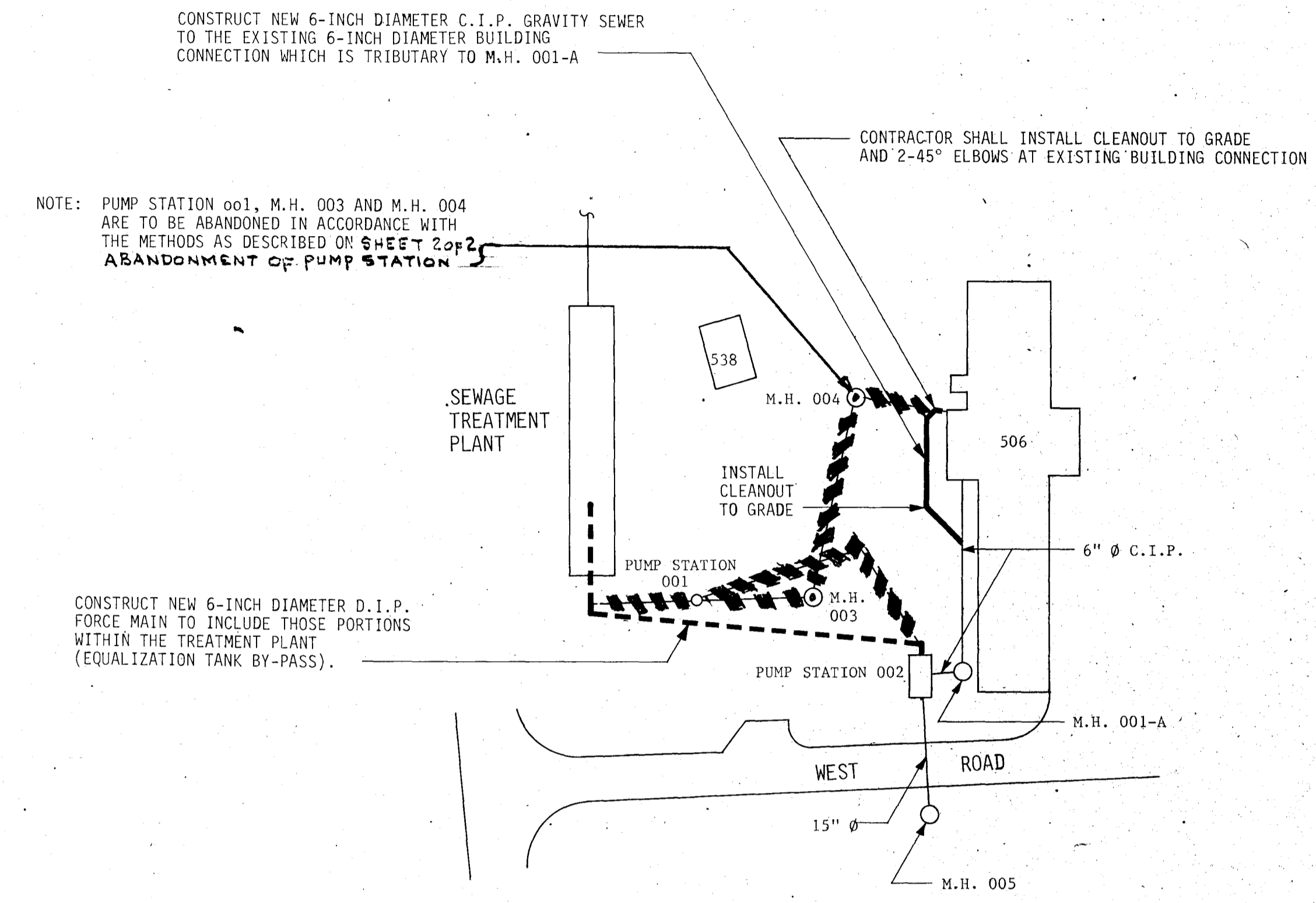
RAW SEWAGE PUMPING STATION MODIFICATIONS
