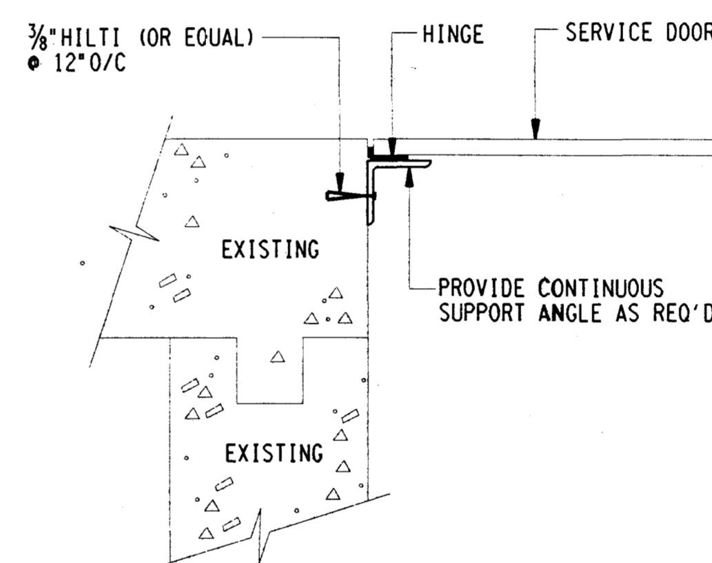
DETAIL 1 NTS
