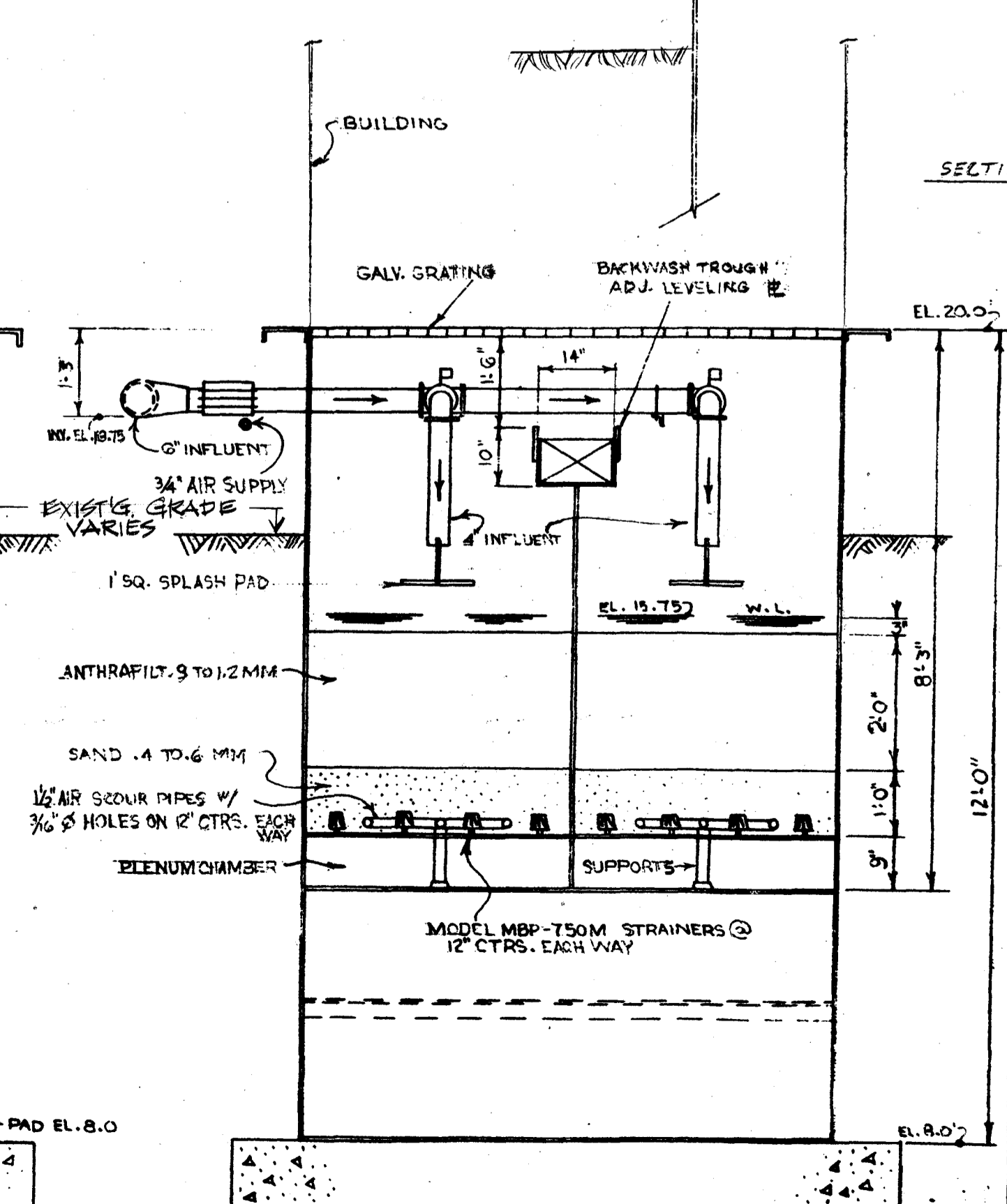
SECTION-CC-
