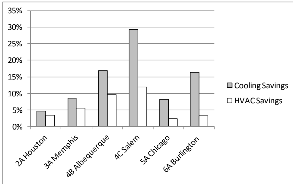
Figure 5: Economizer Savings
