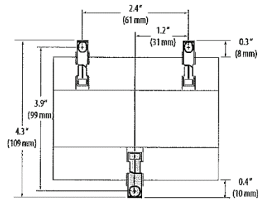
Mounting Diagram
