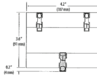
Mounting Diagram
