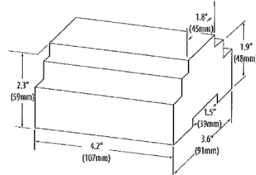
Mounting Diagram
