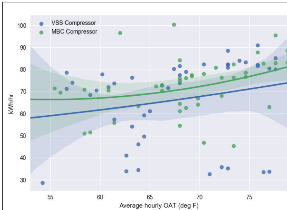
Figure P-4. Energy consumed (in kilowatt-hours) per hour when condenser EWT is between 67.5°F and 72.5°F.
