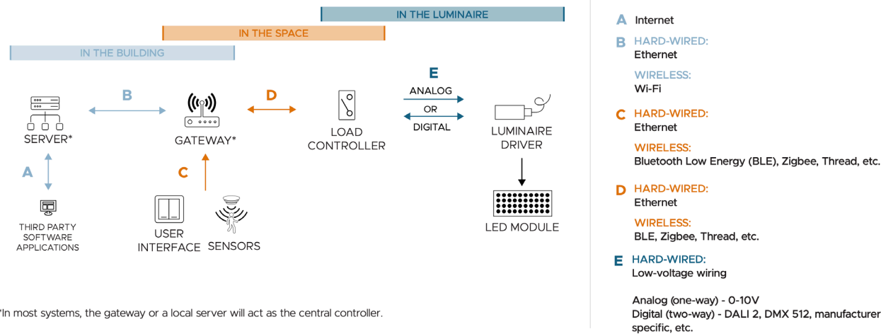
Figure 12 Centrally Networked Control System (Pacific Northwest National Laboratory)
