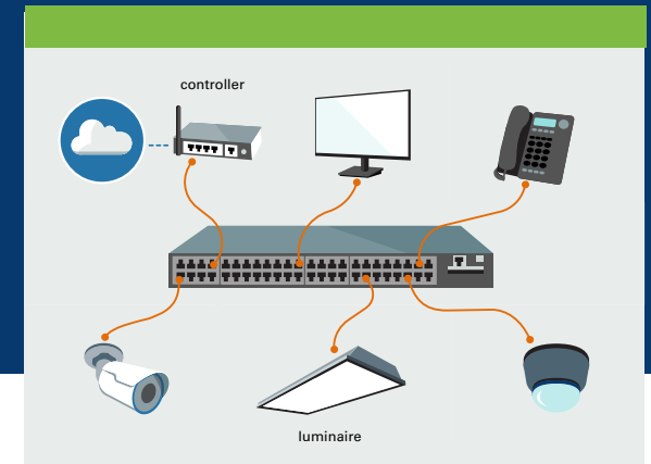
Figure 5 Power-over-Ethernet networks can combine multiple systems (e.g., lighting, security, phone, etc.). At the center is a network switch with ports; orange cables combine power and data.
