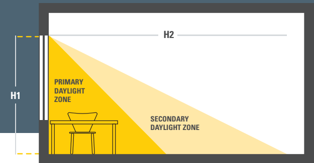
Figure 22 Daylight-Responsive Control Zones
