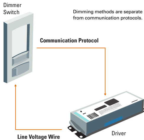
Figure 3 The Driver Determines the Dimming Method
