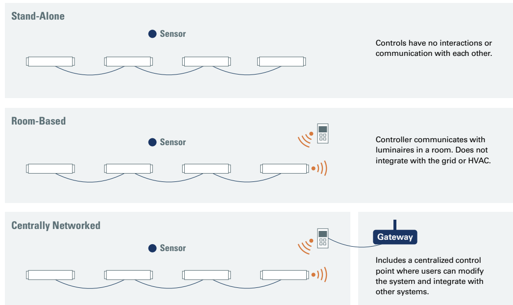
Figure 9 Lighting Controls Configurations
