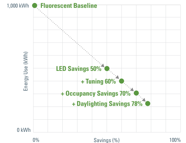
Figure 20 Diminishing Returns for Combined Energy Savings (highlighted in Table 15)
