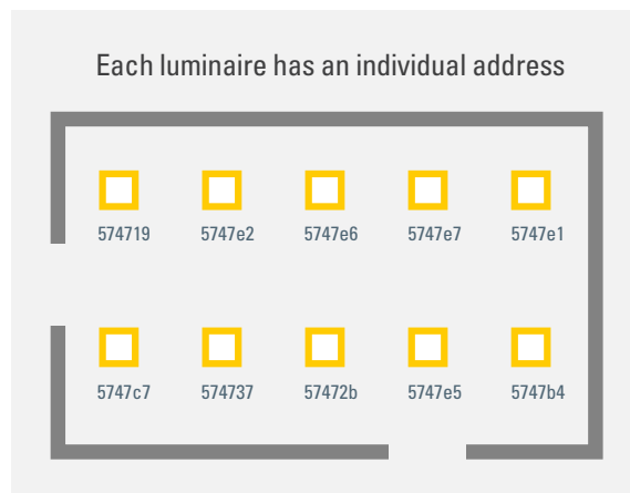
Figure 18 Reflected Ceiling Plan of an Open Office in a GSA Building
