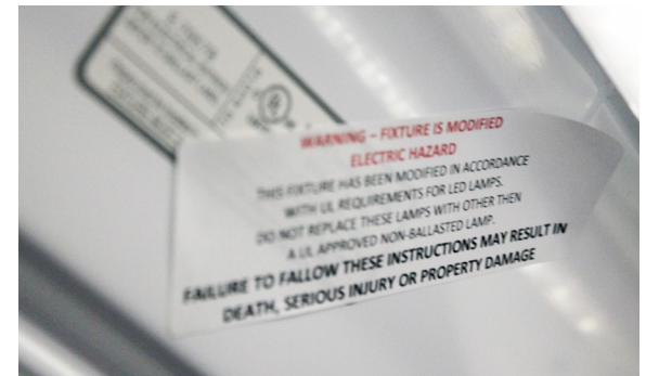
Label indicates the fixture was rewired and that fluorescent tubes should not be installed for safety reasons. Photo credit Michael Myer, PNNL
