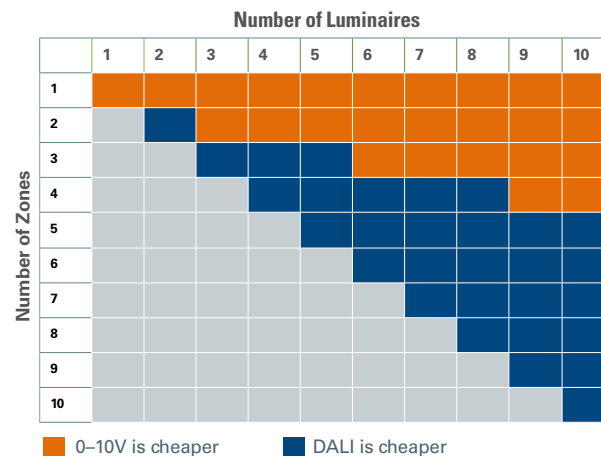
Figure 16 Digital Control is Less Expensive for Multiple Lights / Zones*
