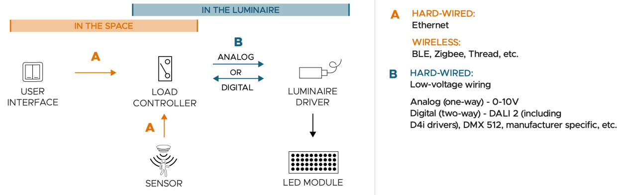
Figure 11 Room-Based Control System (Pacific Northwest National Laboratory)
