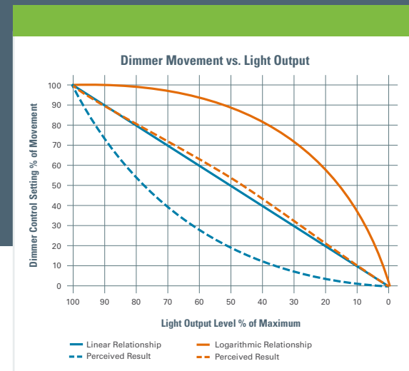
Figure 21 Light Output Compared to Perceived Results for 0–10V and DALI
