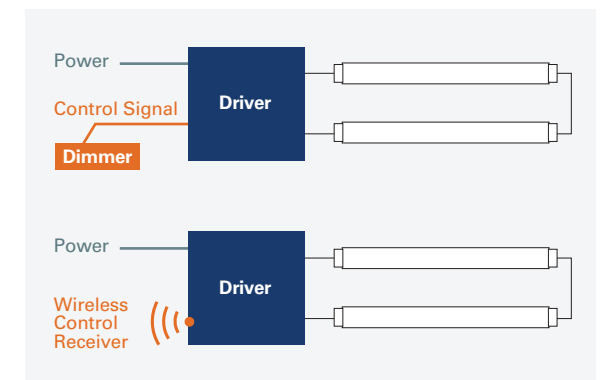
Figure 4 Wired and Wireless Control for Type C TLED
