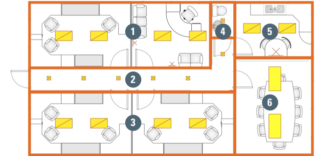
Figure 8 Design Lighting Zones by Fixture Type, Application, and Location
